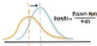
Naïve Bayes
