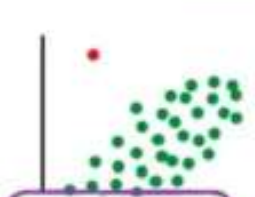
Outliers
