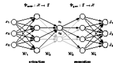
neural network
